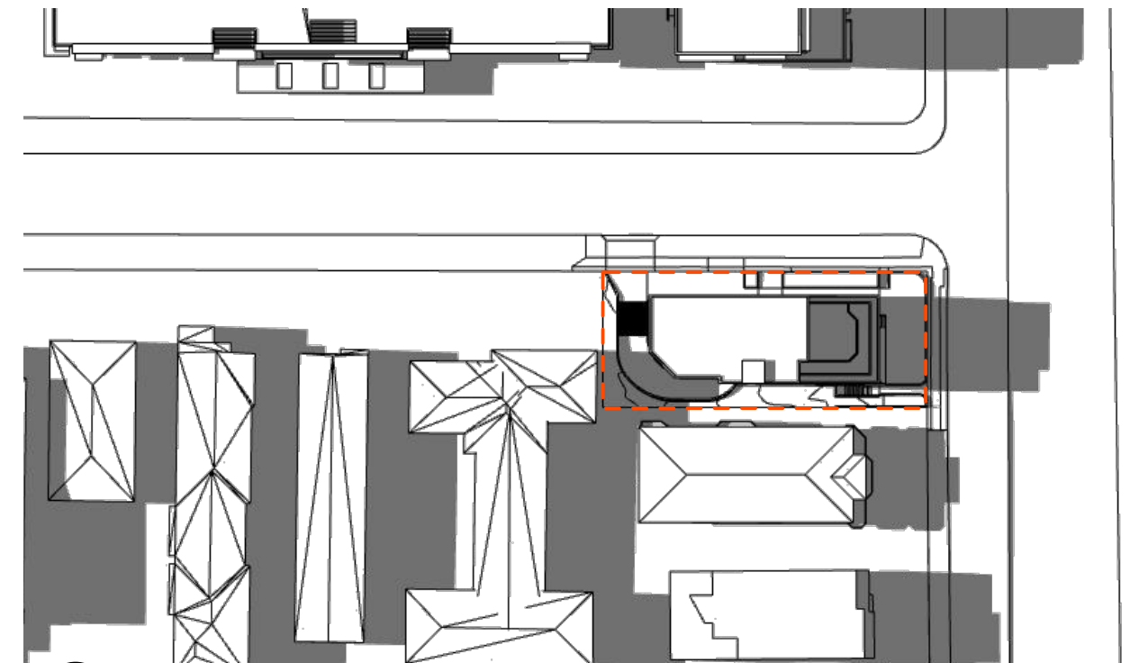
3 SHADOW DIAGRAM 21/03 - 3PM - Scale -
